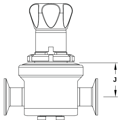
Optional panel mounting
