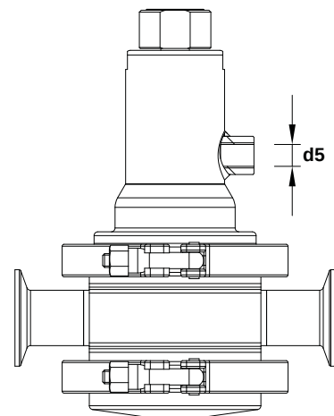
Optional leakage line connection
