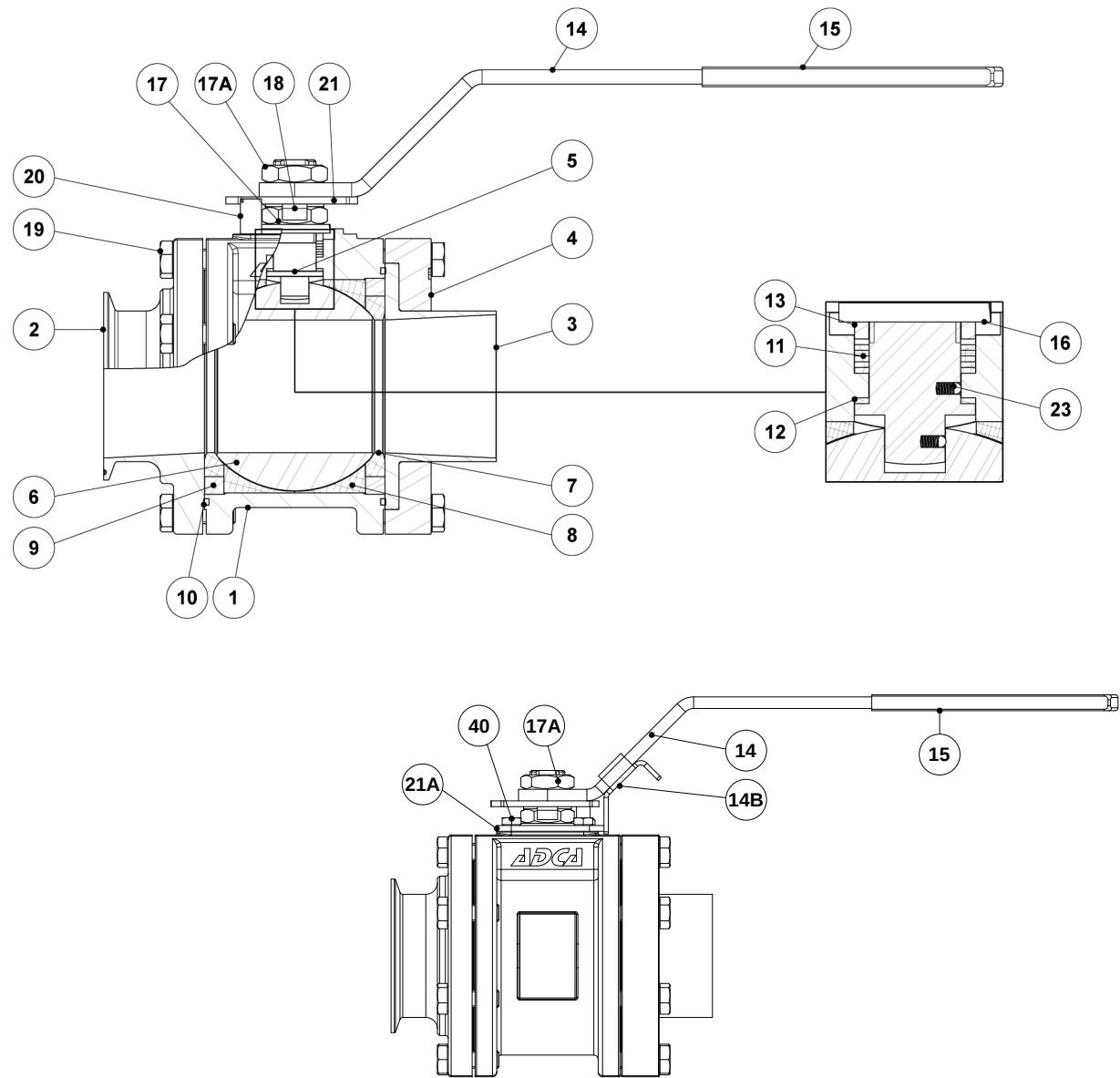
Optional flat lever with locking system
