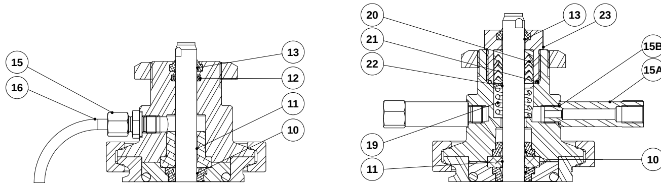
Optional steam barrier
