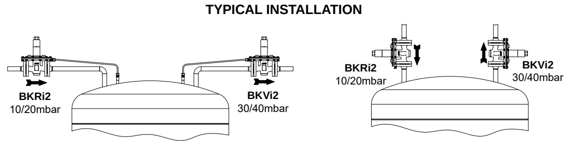
Blanketing with overpressure
