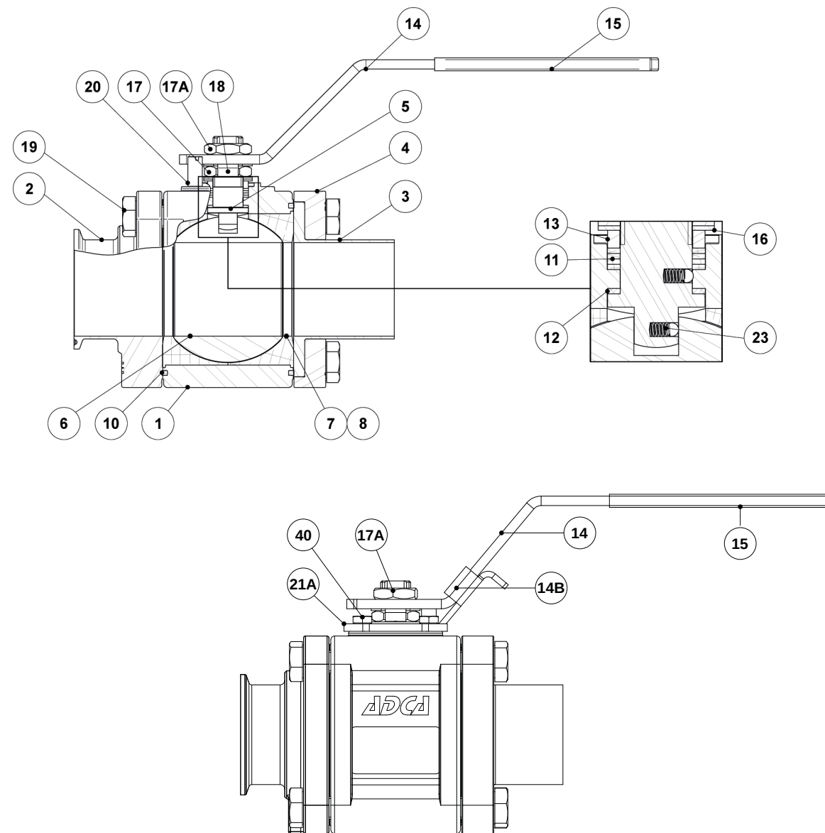
Optional flat lever with locking system
