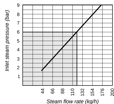
CAPACITY CHART
