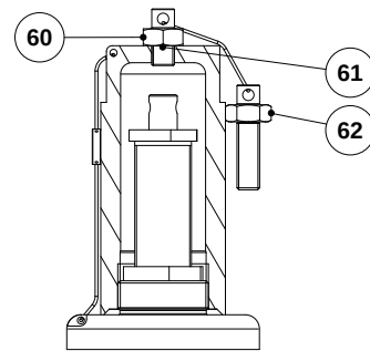
Optional blocking system
