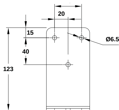
Optional wall mounting
