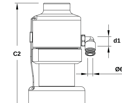
Optional pneumatic lifting device
