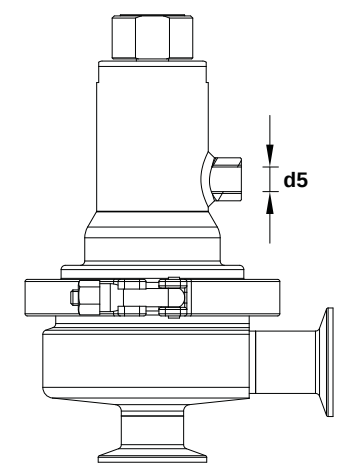
Optional leakage line connection
