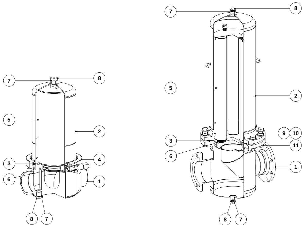
1/4" to 3" – DN 10 to DN 80
