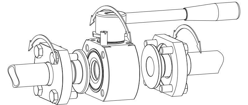
Tube weld easy and quick installation
