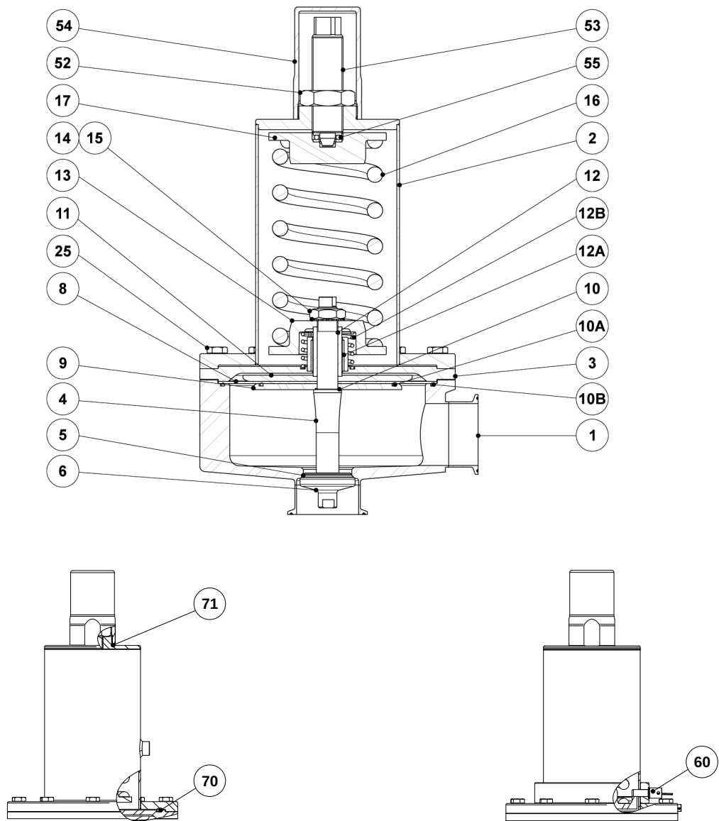
Optional leakage line connection
